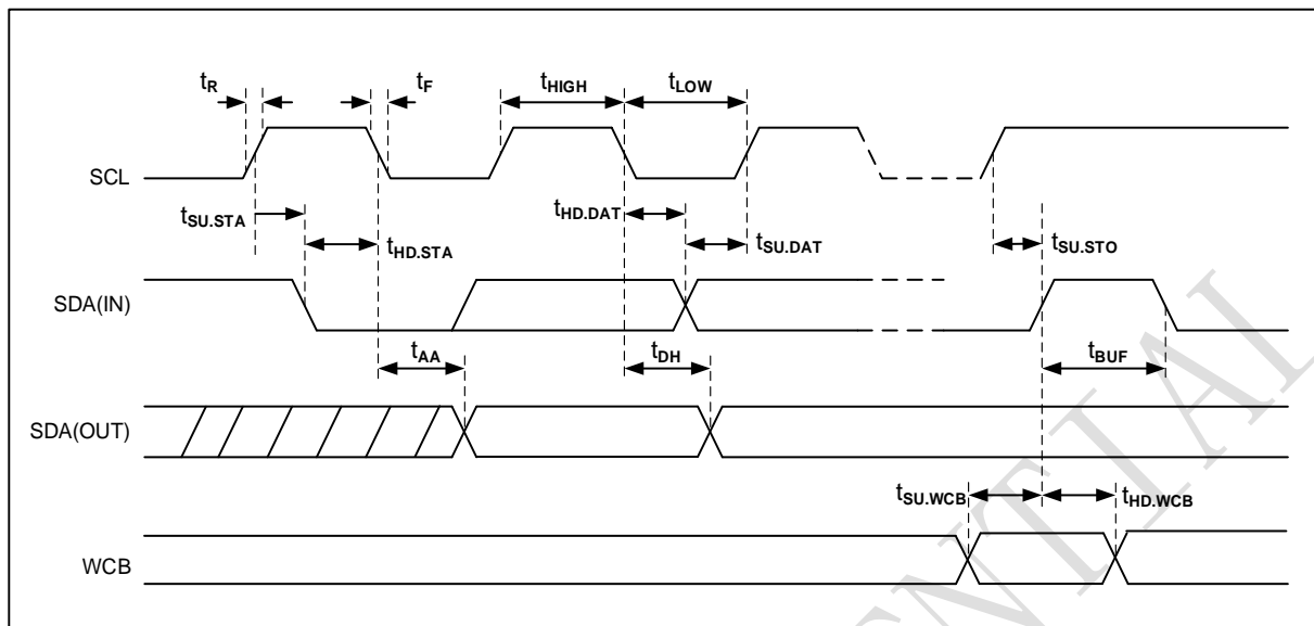
Figure 3-1 Bus Timing
