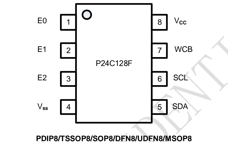
Figure 1-1 Pin Configuration
